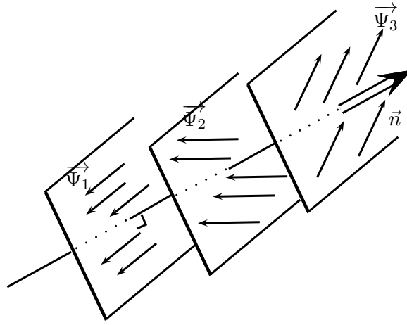
FIGURE 3 – Onde vectorielle \vec{\Psi}(M, t_0) plane (dans le cas particulier transverse )
