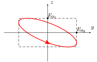
FIGURE 13 - \varphi \in [\frac{\pi}{2}, \pi]
