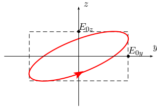
FIGURE 11 - \varphi \in [0, \frac{\pi}{2}]
