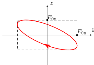
FIGURE 15 - \varphi \in [\pi, \frac{3\pi}{2}]
