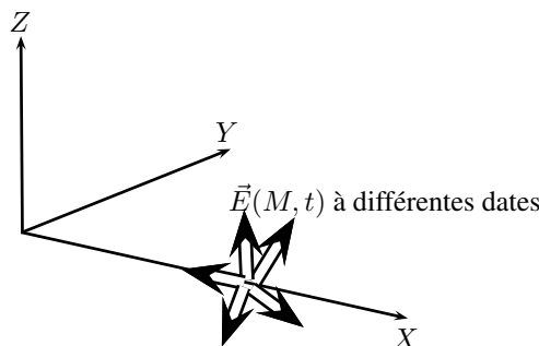
FIGURE 18 – Lumière naturelle
