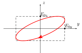
FIGURE 17 - \varphi \in [\frac{3\pi}{2}, 2\pi]
