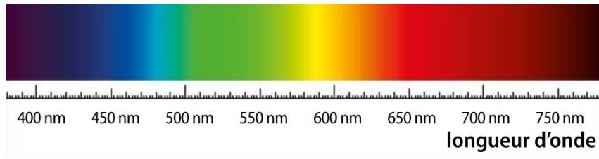
FIGURE 2 – Spectre visible
